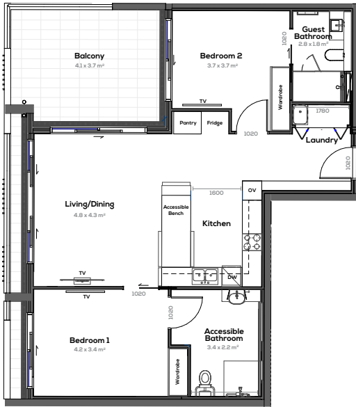
Floor plan of 2 bedroom apartment.
